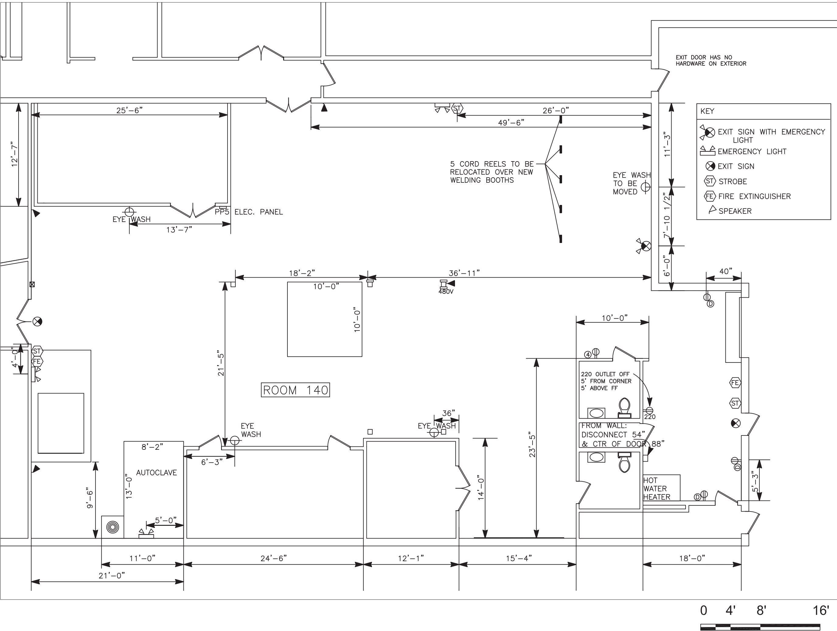
NEW WELDING LAB AT ROCHESTER GBCC EXISTING CONDITIONS
