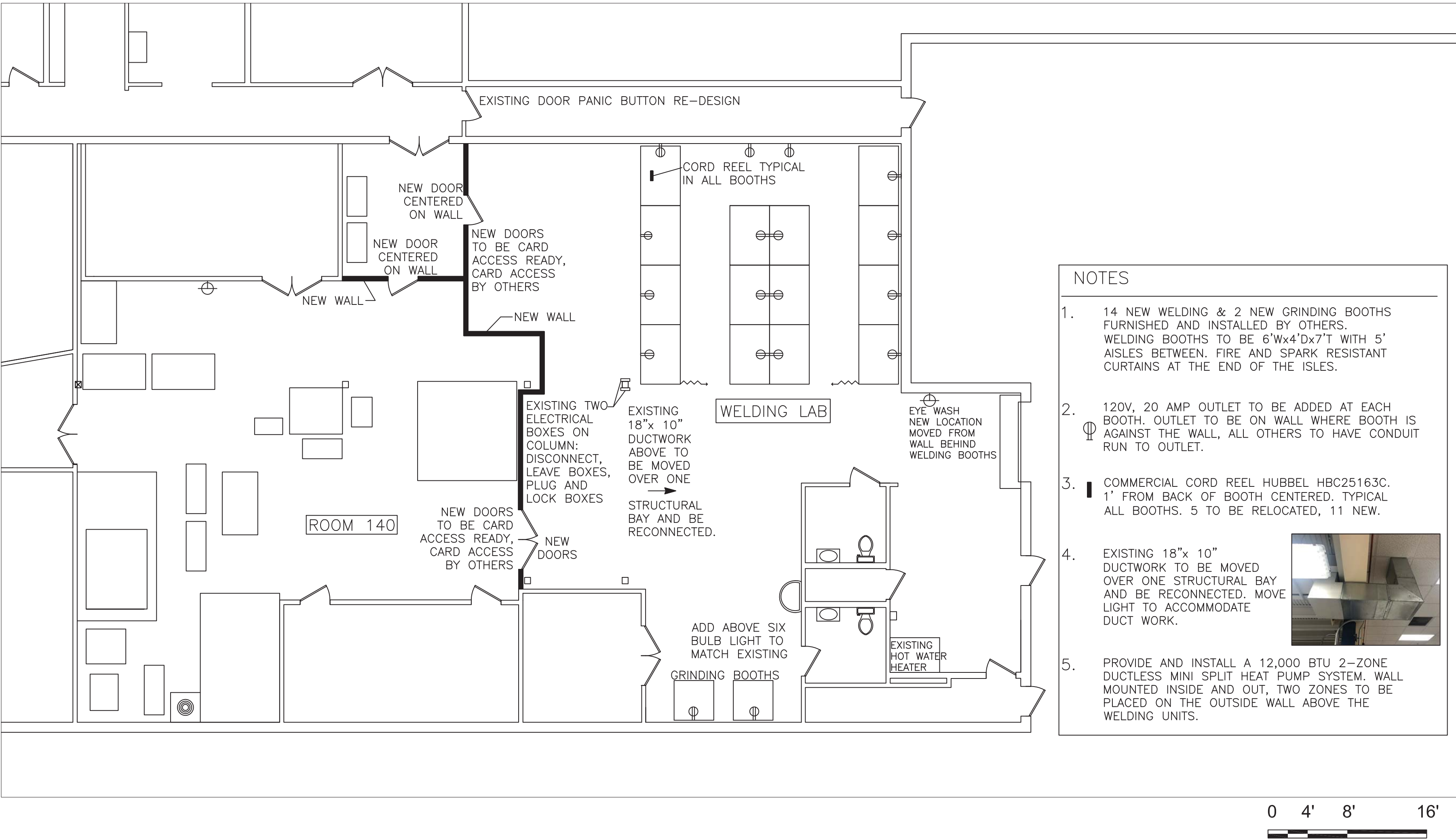
NEW WELDING LAB AT ROCHESTER GBCC NEW WORK
